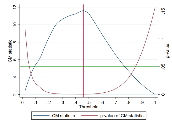
Figure 14: CM statistic for the deposit rate
