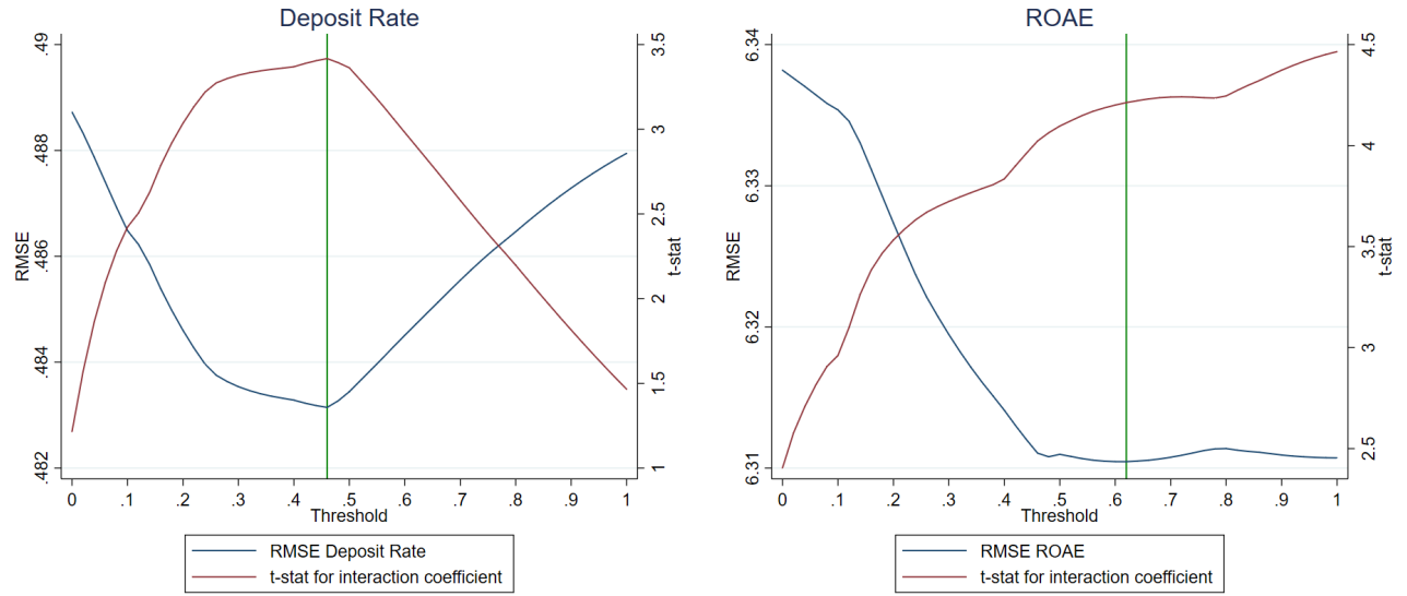
Figure 11: RMSE for threshold tests
